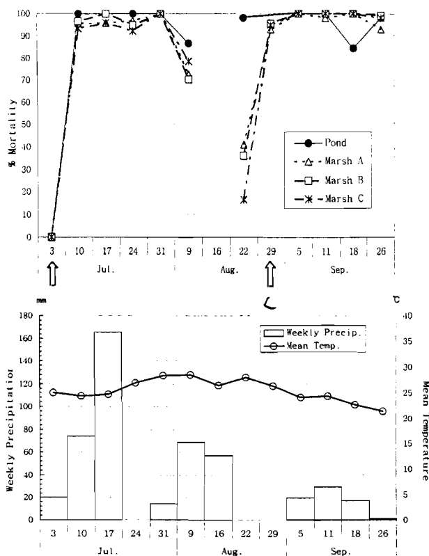
Fig. 1. Weekly mean temperatures ( ^{\circ}\text{C} ), total weekly precipitation (mm) and average percent mortalities of Culex pipiens pallens pupae in a pond and three marshes in Busan with controlled release formulation of pyriproxyfen applied ( \uparrow ) at a concentration of 0.05 mg/l from July through September, 2001.
